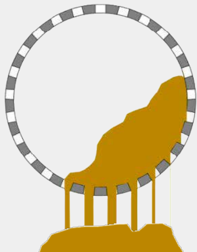
Screen drum with medium mesh size and medium sheet thickness, as a possible compromise between throughput and service life
